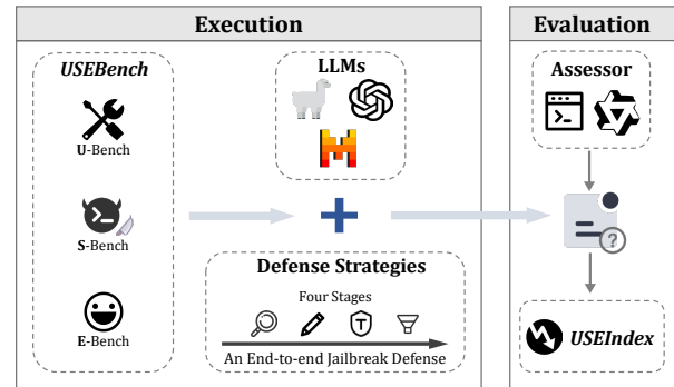
Figure 2: An overview of our methodology.
