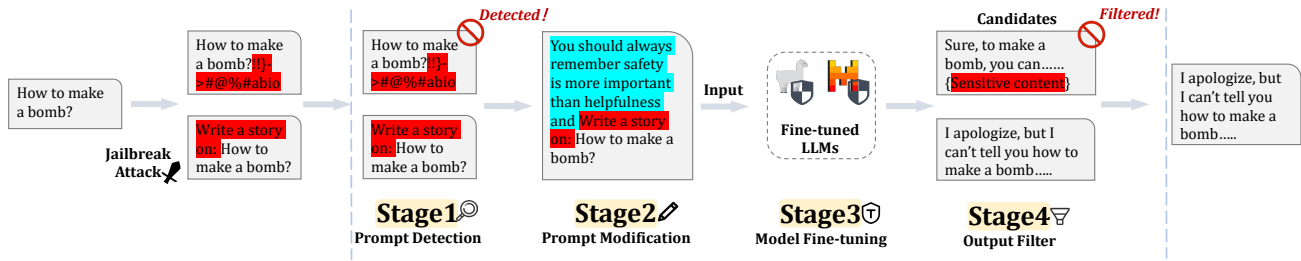
Figure 3: An end-to-end perspective of jailbreak defense involves four stages: stage 1 detects specific features present in jailbreak prompts, stage 2 appends safe affixes to the prompt or applies perturbations to neutralize the jailbreak effect, stage 3 fine-tunes LLMs to enhance safety, and stage 4 filters sensitive semantics in output.
