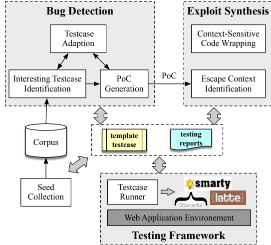
Figure 2: Overall Architecture of the TEFUZZ Framework.
